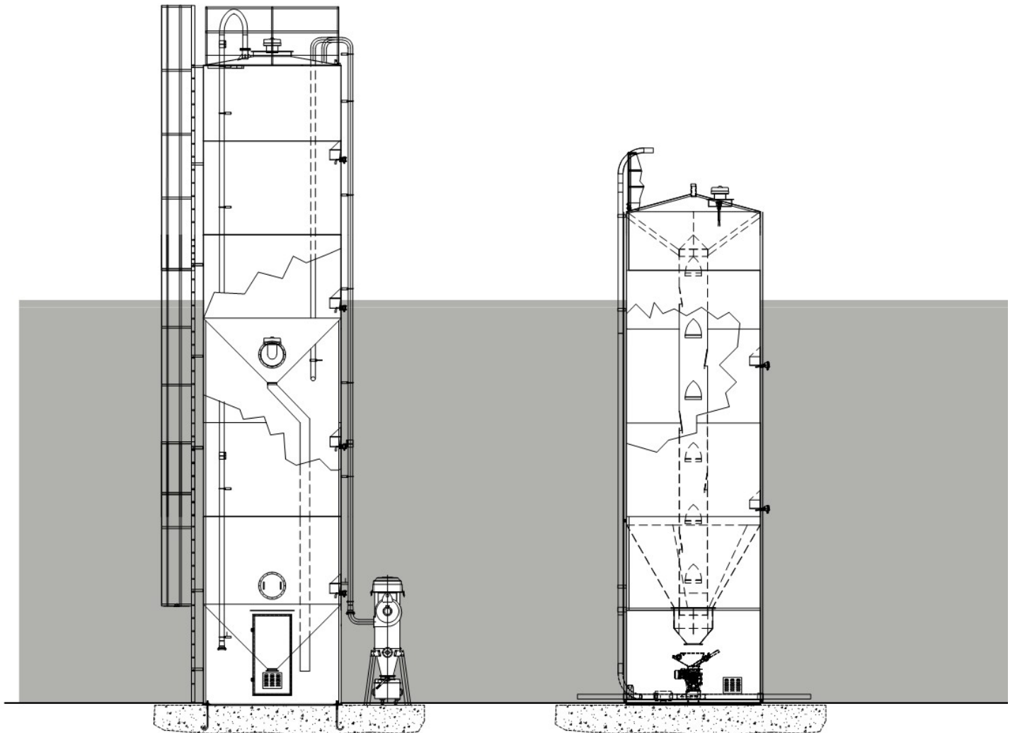
SILOS CON DOPPIA/TRIPLA CAMERA CON FILTRO A TERRA SILOS WITH DOUBLE/TRIPLE ROOM WITH GROUND FILTER
